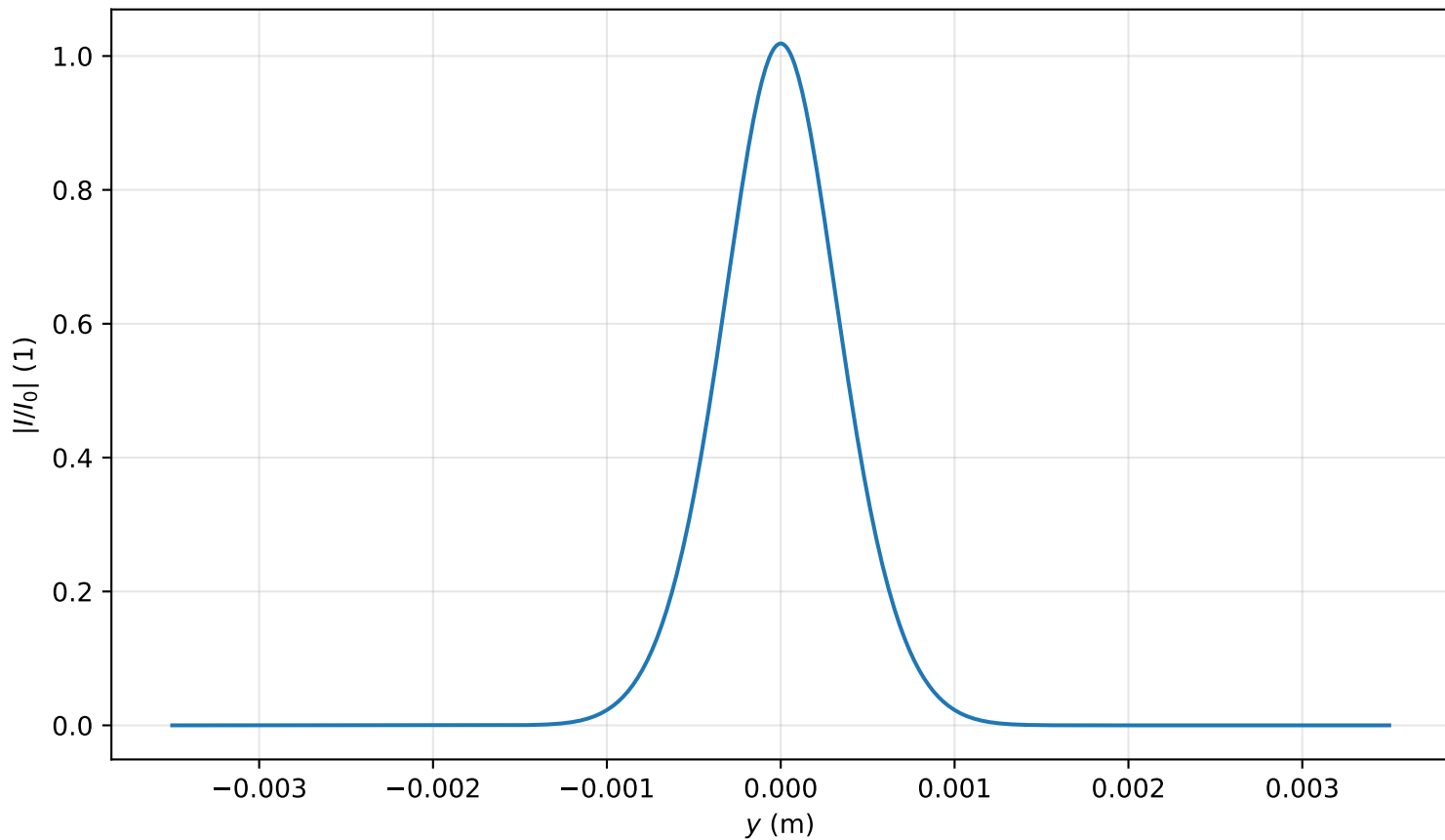
Intensity profile I(x=0, y, z=0.716)/I_0 , P_{in}=0.4P_{cr} , artificial time
